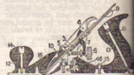
Sectional View of Bailey Iron Plane
