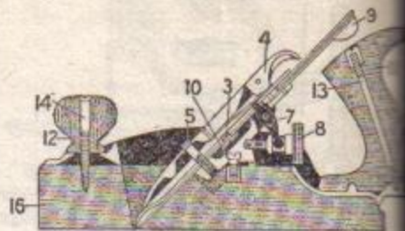
Sectional View of Bailey Wood Plane
